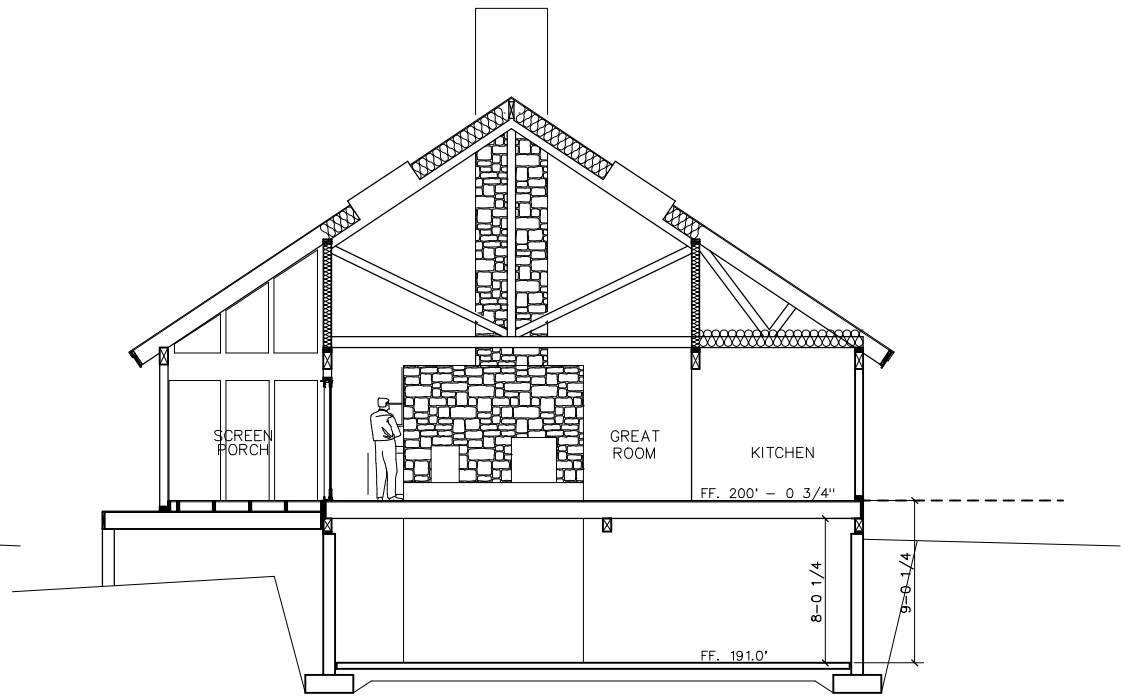
B-B SECTION
